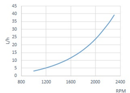
Fuel consumption
