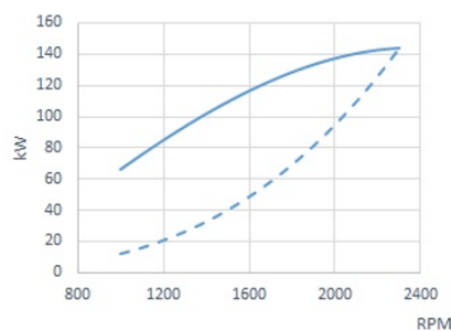
Power (ISO 3046/1)
