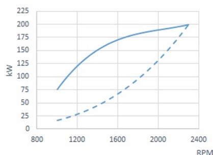
Power (ISO 3046/1)
