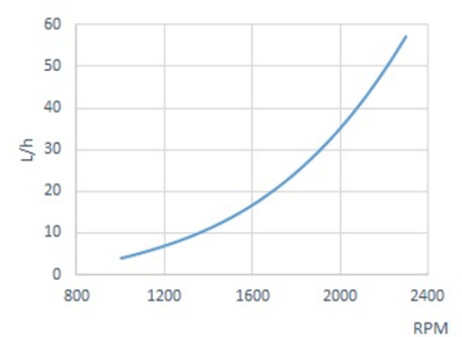
Fuel consumption
