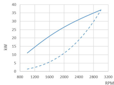
Power (ISO 3046/1)
