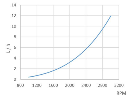
Fuel consumption
